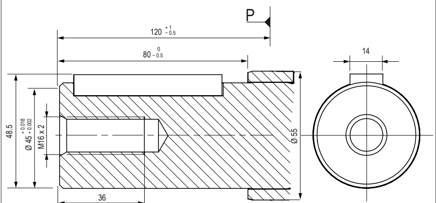
D1 Zylindrische Welle \varnothing 45 DIN 6885 AS 14 x 9 x 63
