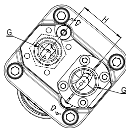
VIEW G
