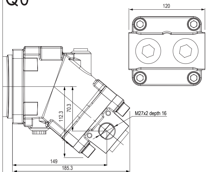
Q0 Side threaded ports A and B
