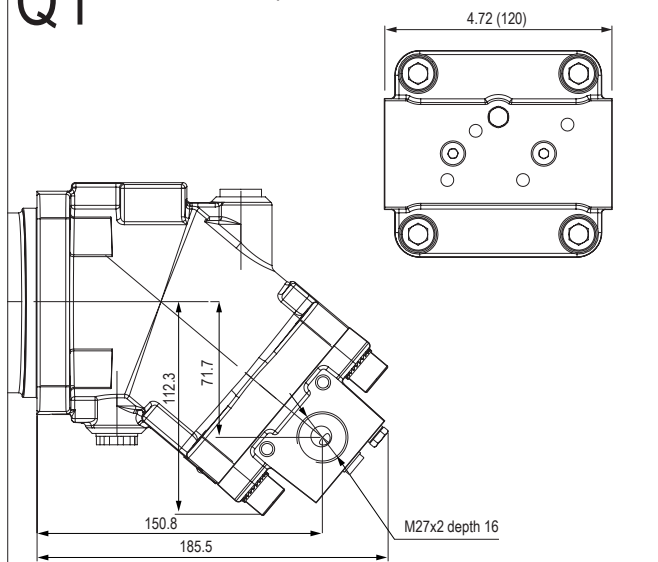
Q1 Side threaded ports A and B
