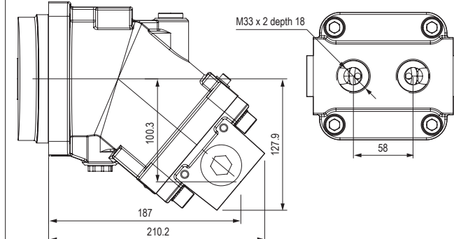
Q1 Side threaded ports A and B
