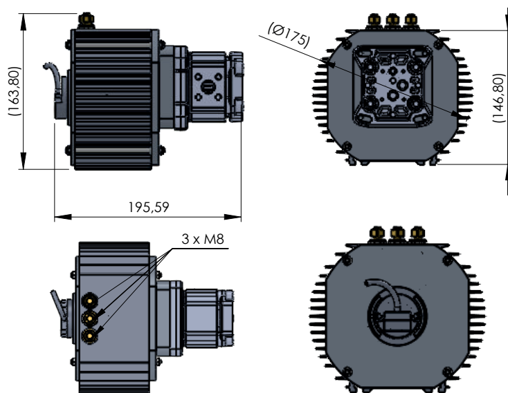
External gear - 3,07cc.
