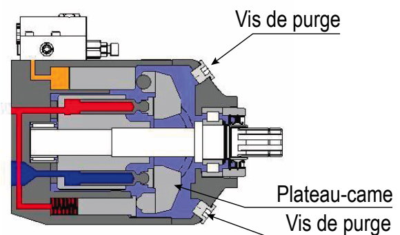
Figure 2 - Cylindrée nulle
