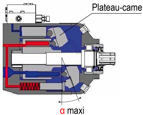
Figure 1 - Cylindrée maxi
