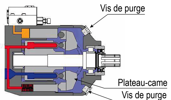
Figure 2 - Cylindrée nulle
